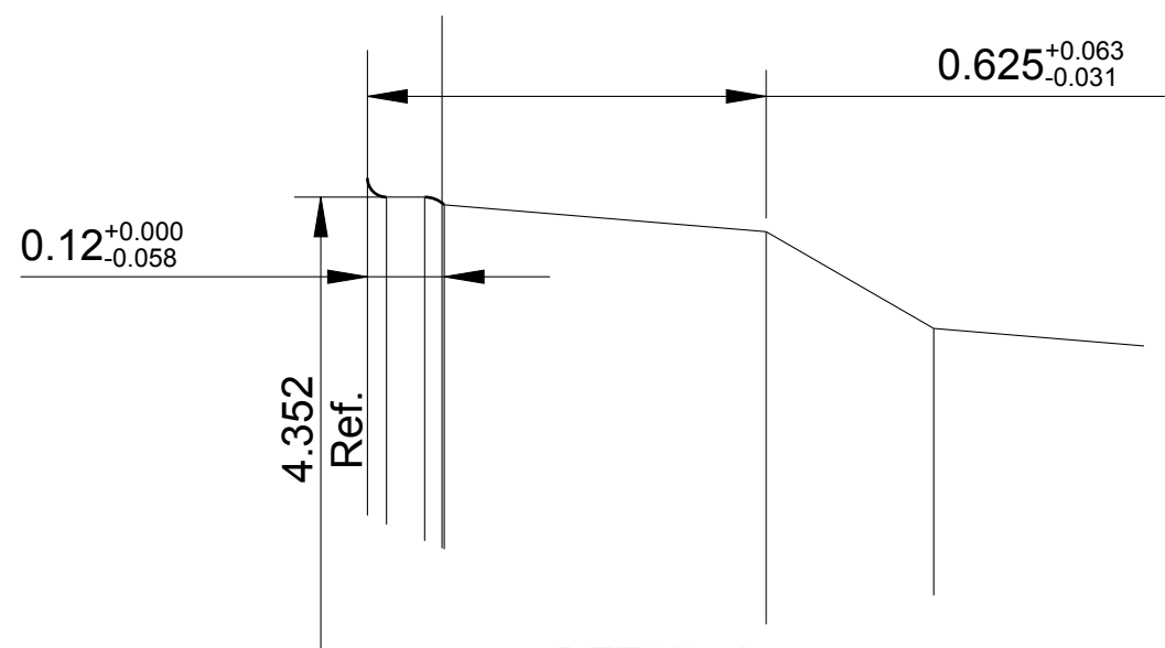
DETAIL A SCALE 3.000
